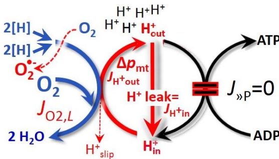
Fig. 5. LEAK state when phosphorylation is arrested: J_{\gg p} = 0 , and oxygen flux, J_{O_2,L} , is controlled mainly by the proton leak, which equals J_{H^+,in} , at maximum \Delta p_{mt} (see also Fig. 2).
