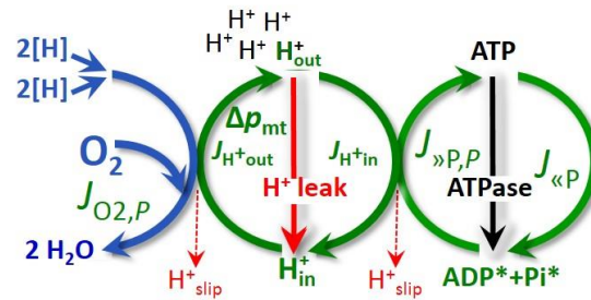
Fig. 3. OXPHOS state when phosphorylation, J_{»P,P} , is supported by a high \Delta p_{mt} , is stimulated by kinetically saturating [ADP]^* and inorganic phosphate, [Pi]^* . O_2 flux, J_{O_2,P} , is highly coupled at a maximum \gg P/O_2 ratio, J_{»P,P}/J_{O_2,P} (see See also Fig. 2.).
