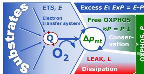
Fig. 6. Four-compartmental model of oxidative phosphorylation with respiratory states (ETS, OXPHOS, LEAK) and corresponding rates ( E , P , L ). Modified from Gnaiger (2014).
