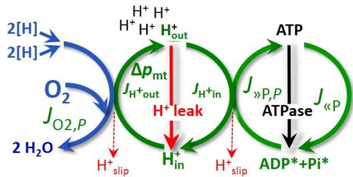
Fig. 3. OXPPOS state when phosphorylation, J_{»P} , is supported by a high \Delta p_{mt} , is stimulated by kinetically saturating [ADP]^* and inorganic phosphate, [Pi]^* . O_2 flux, J_{O_2,P} , is highly coupled at a maximum \gg P/O_2 ratio, J_{»P,P}/J_{O_2,P} (see also Fig. 2).
